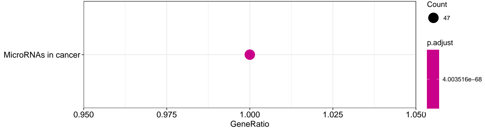
dotplot for kegg
